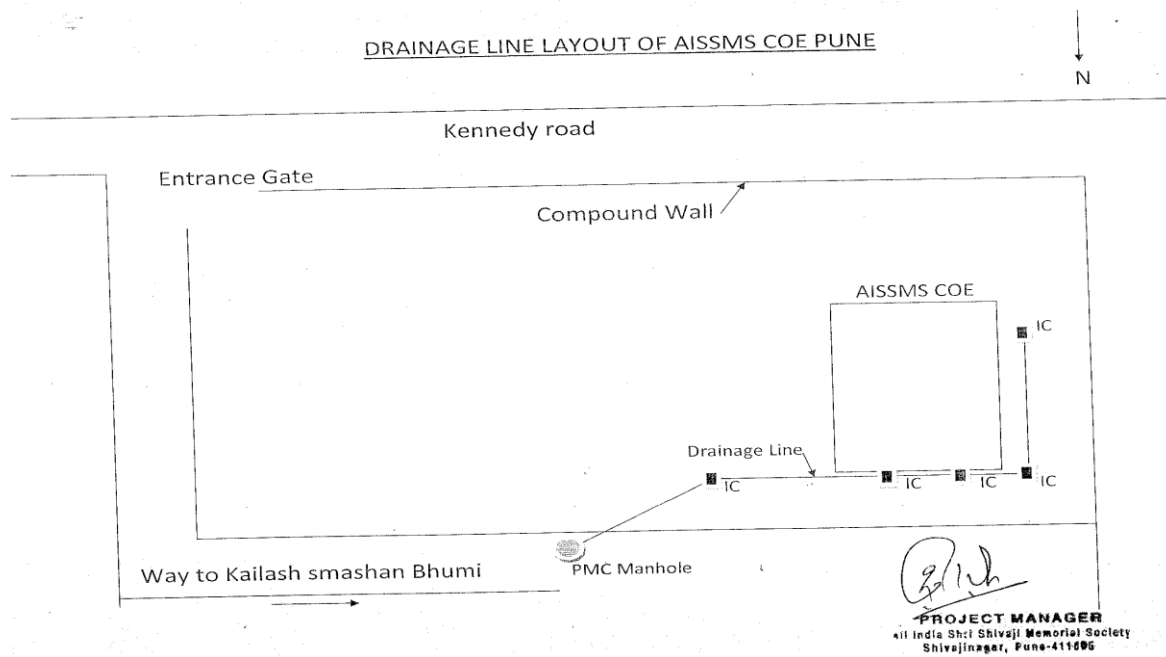
Drawing of Drainage Line of college connected to corporation line.
